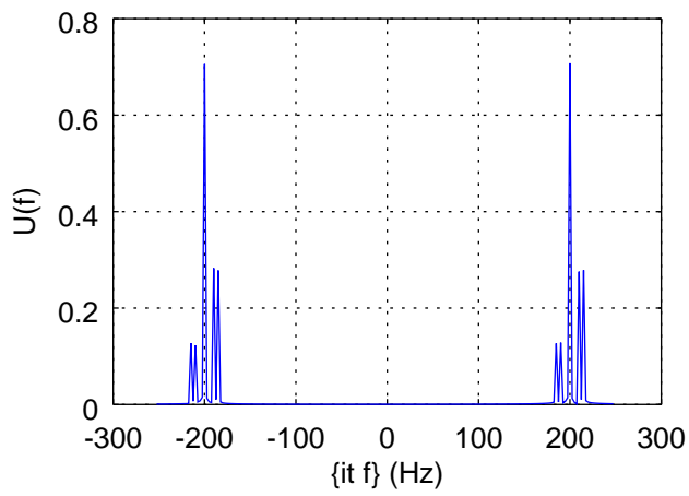
Modulated Signal
