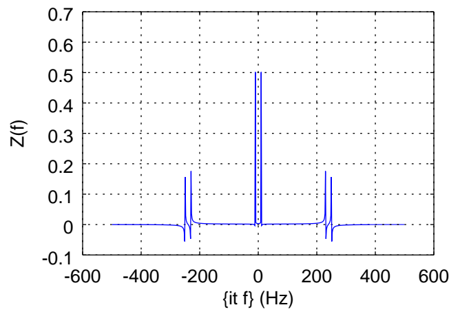
Demodulated Signal
