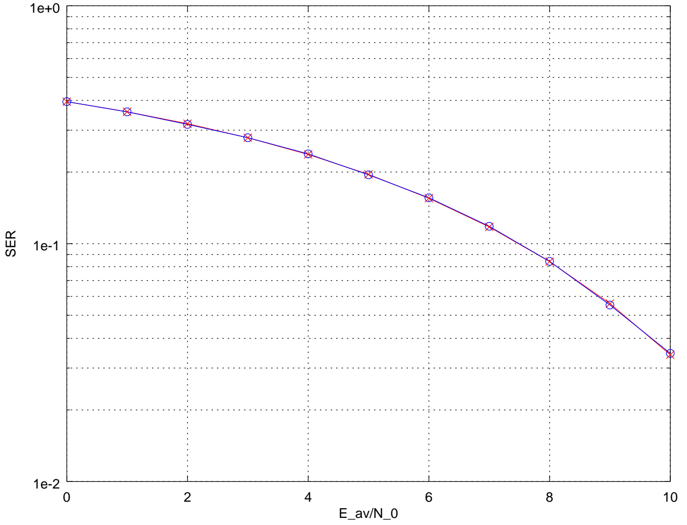
4-PAM over AWGN channel
