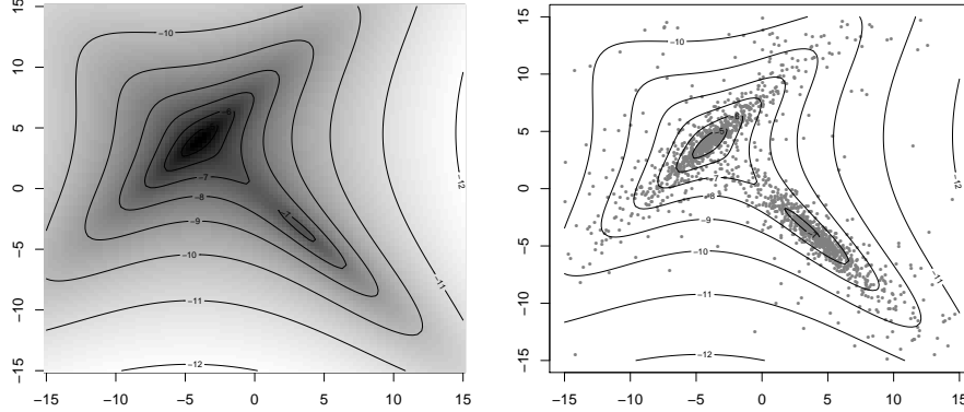
Figure 1: Two-dimensional Gaussian mixture model. Probability density function is depicted on the left and 2000 element sample is depicted on the right.
